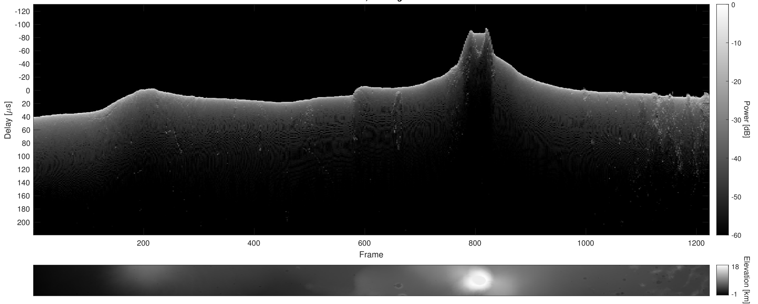
Orbit 7216, Cluttergram
