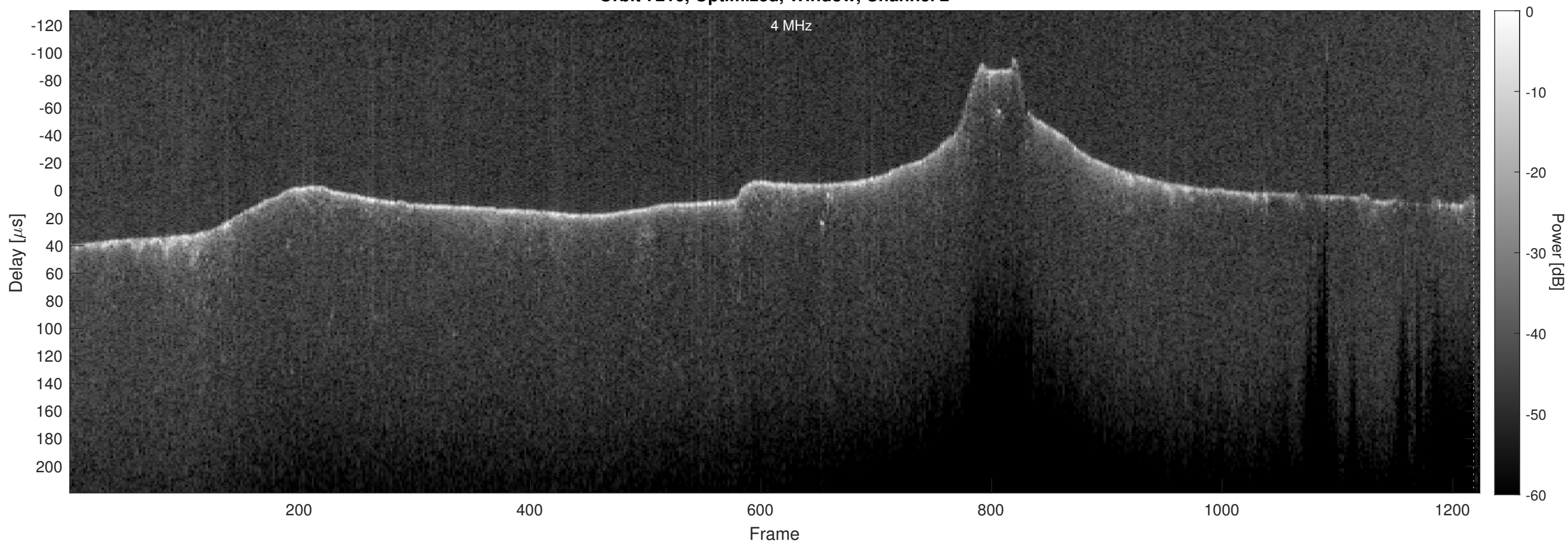
Orbit 7216, Optimized, Window, Channel 2
