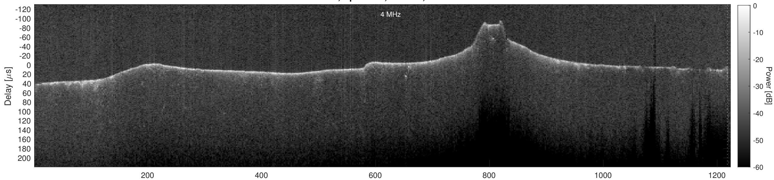
Orbit 7216, Cluttergram
