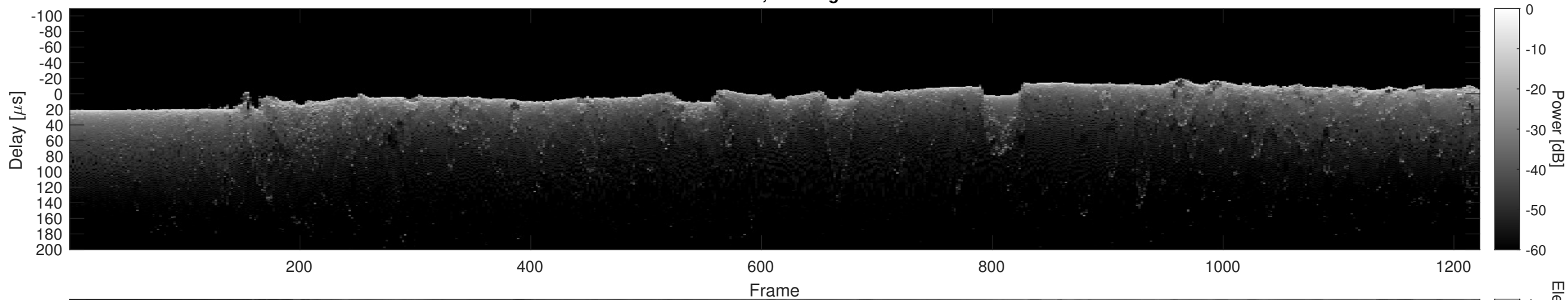
Orbit 7218, Cluttergram
