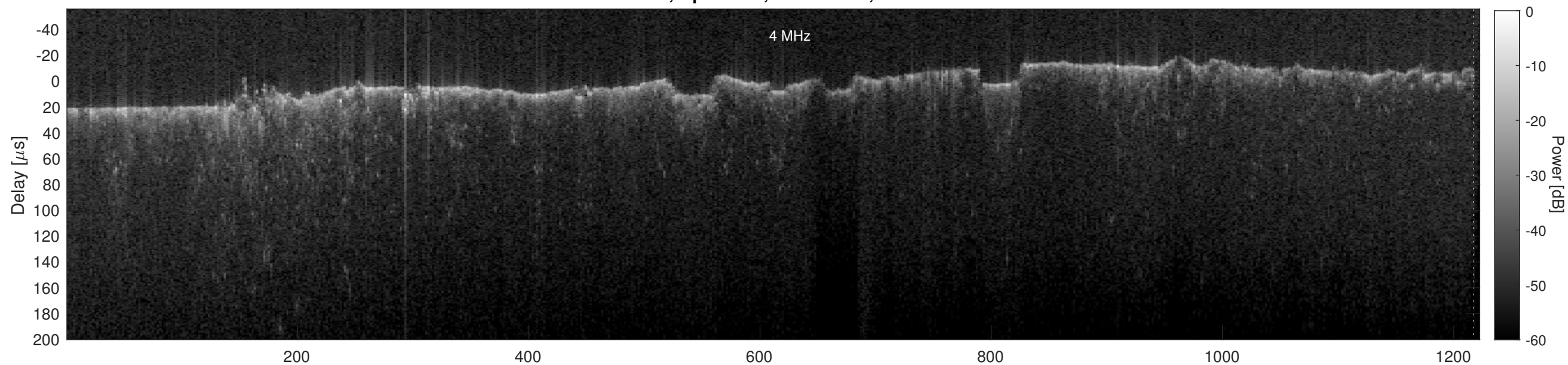
Orbit 7218, Cluttergram
