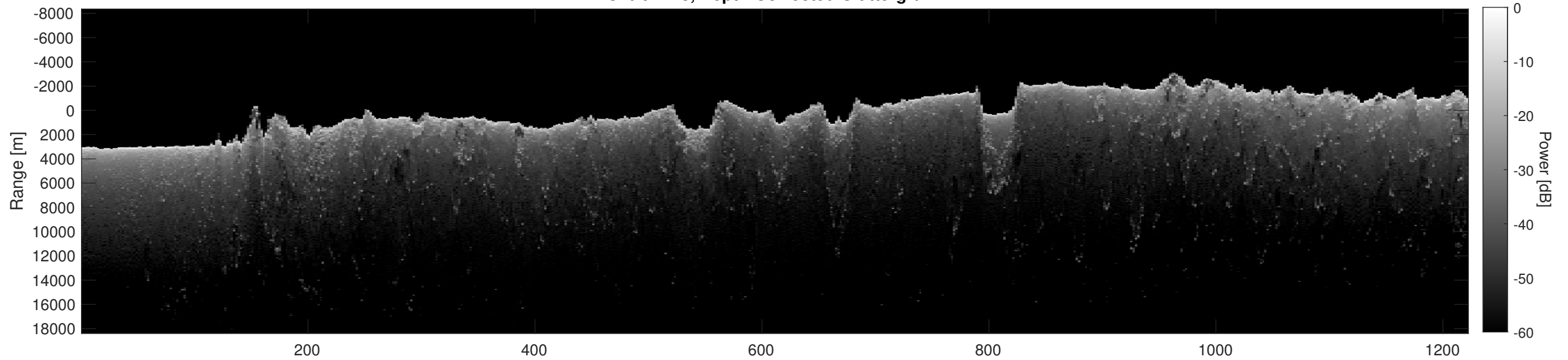
Orbit 7218, Depth-Corrected Cluttergram
