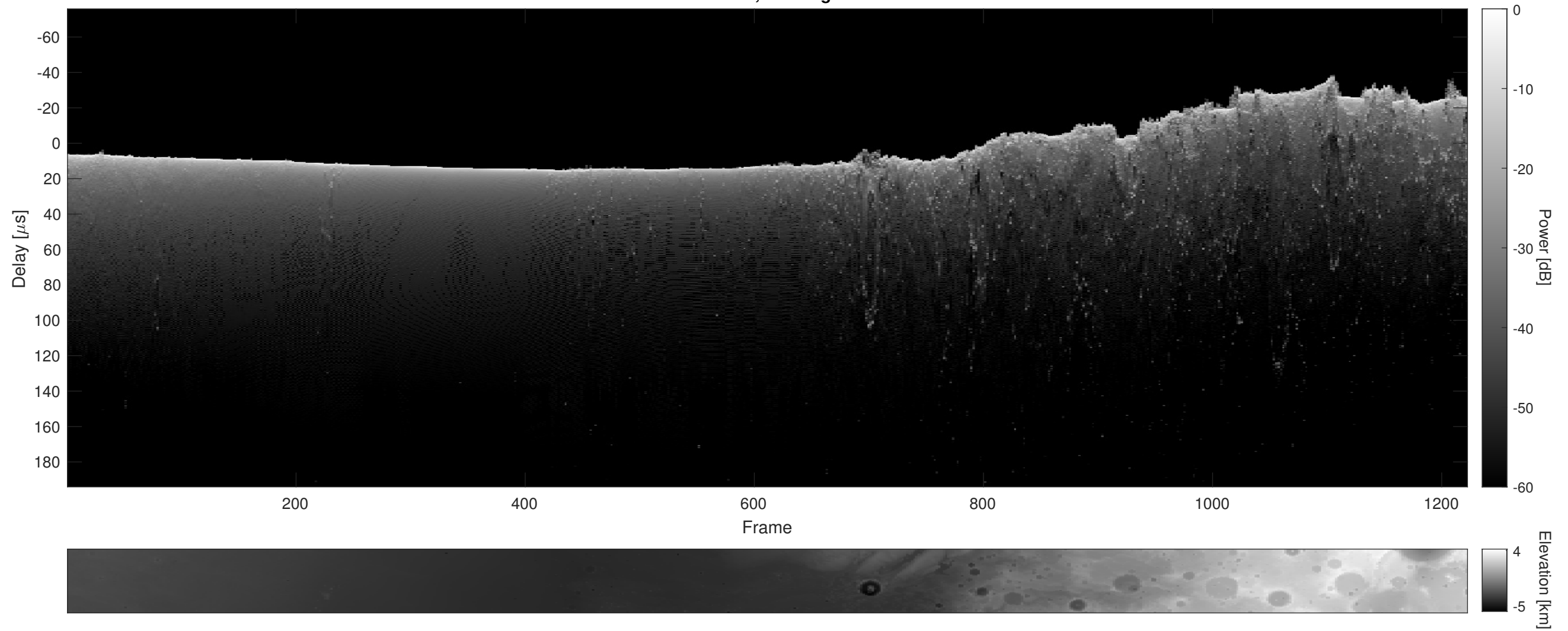
Orbit 7220, Cluttergram
