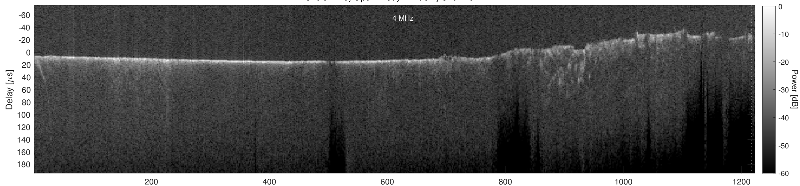
Orbit 7220, Cluttergram
