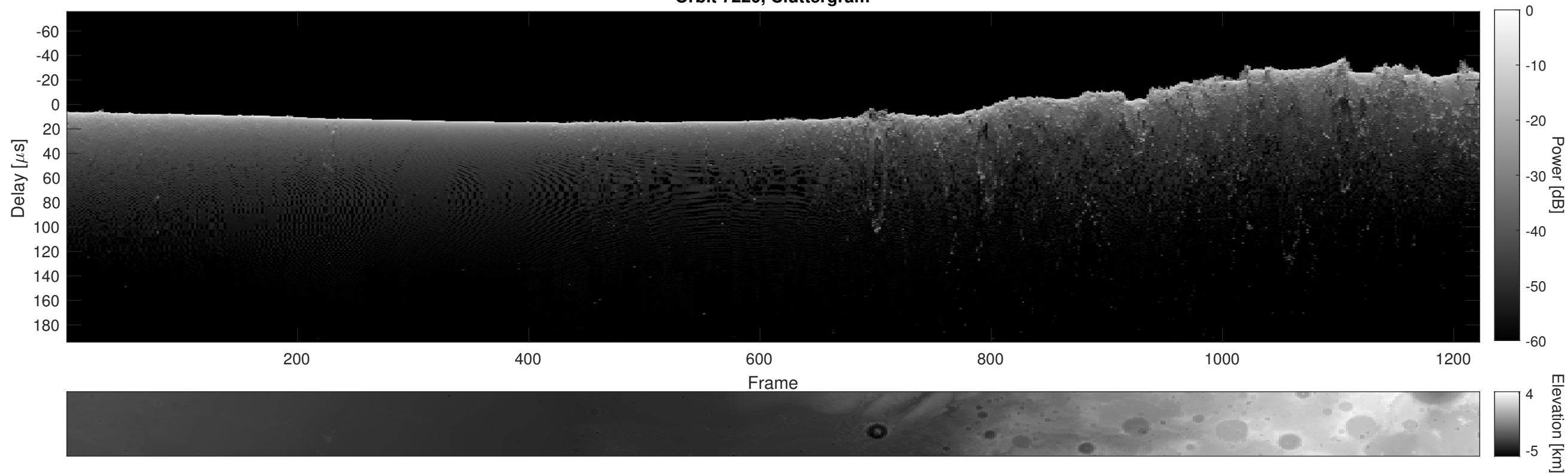
Orbit 7220, Cluttergram
