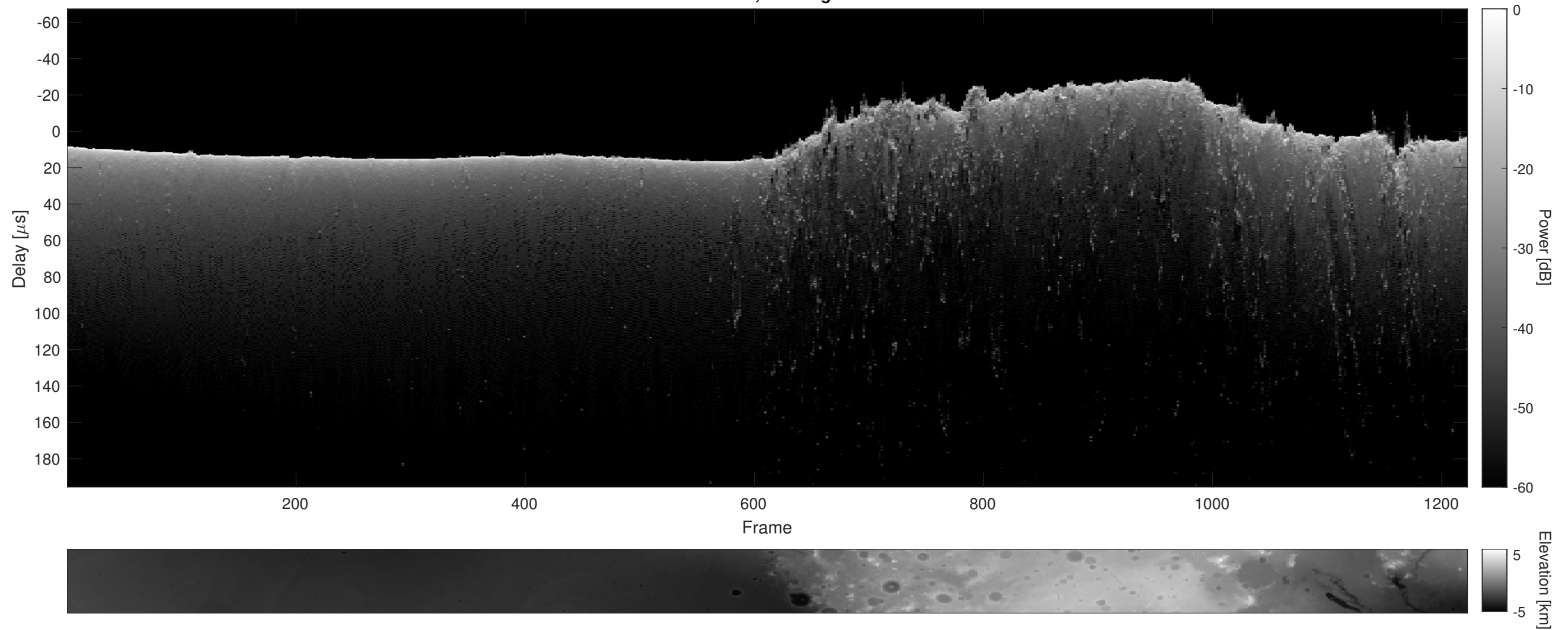
Orbit 7221, Cluttergram
