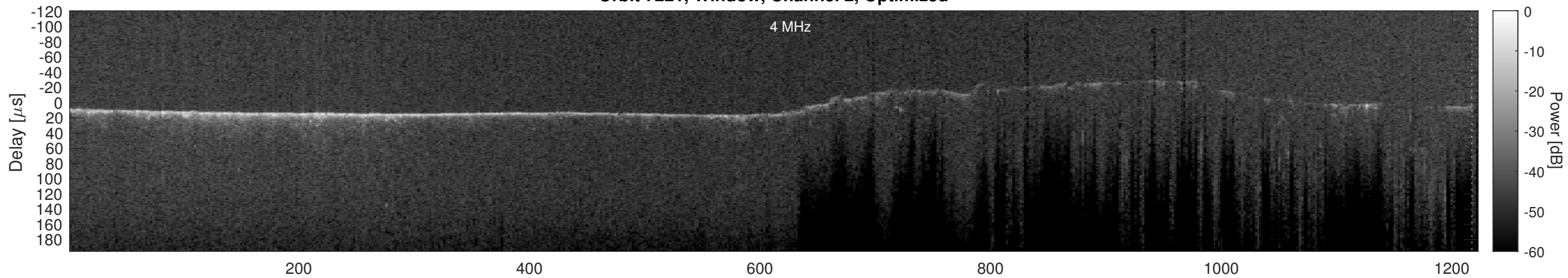
Orbit 7221, Cluttergram
