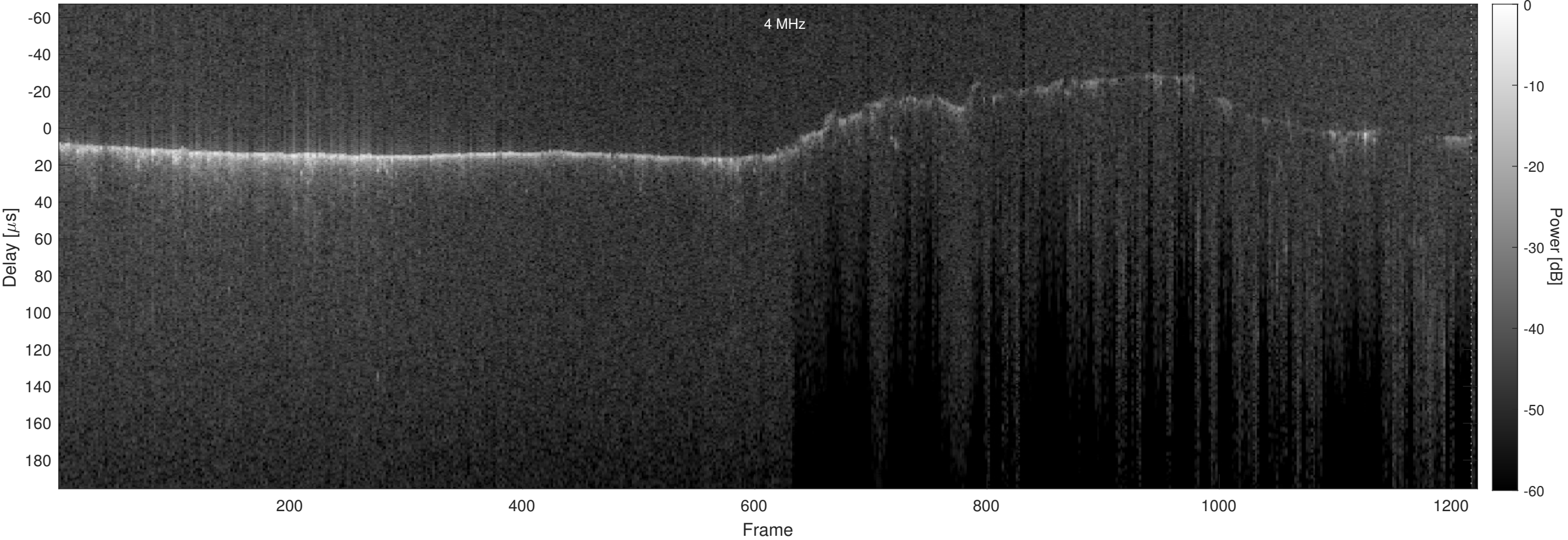
Orbit 7221, Optimized, No Window, Channel 2
