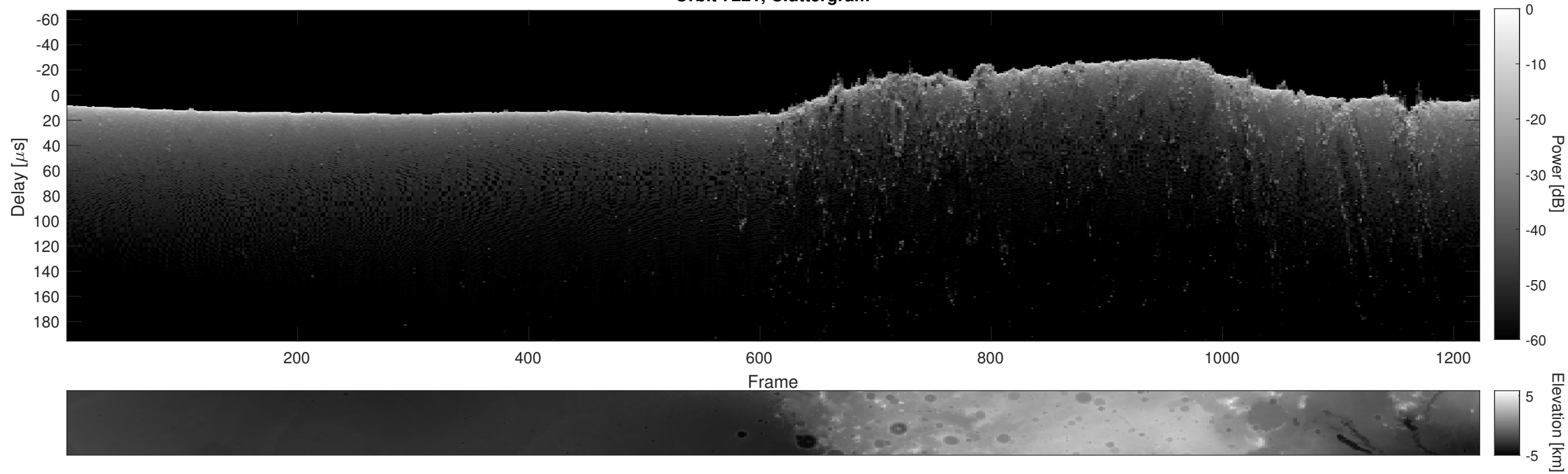
Orbit 7221, Cluttergram
