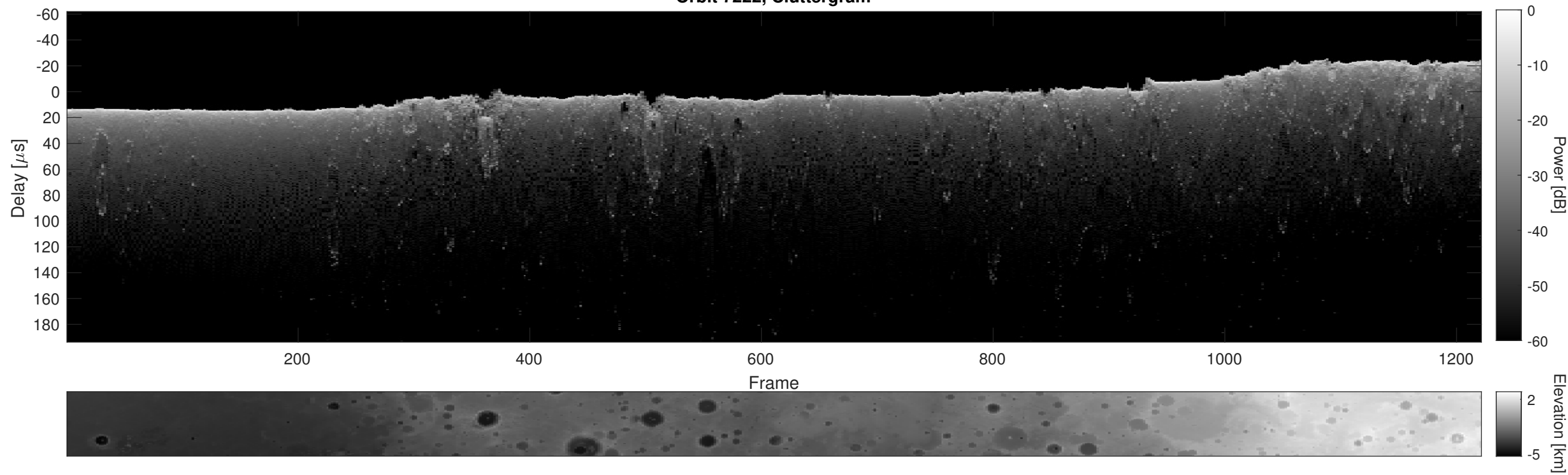
Orbit 7222, Cluttergram
