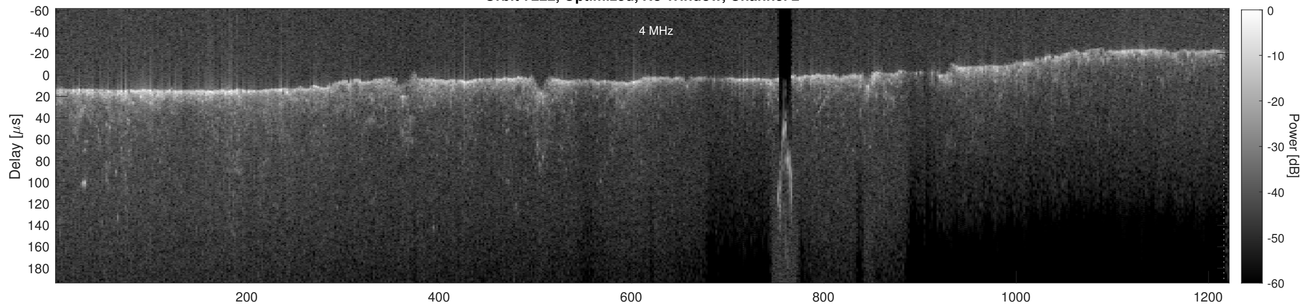
Orbit 7222, Cluttergram
