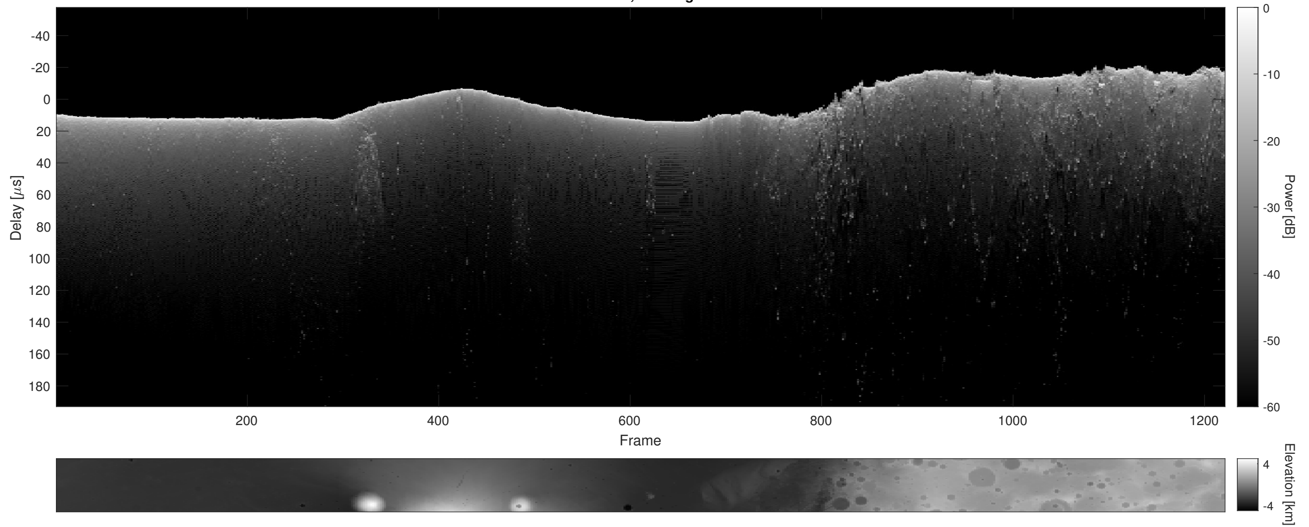
Orbit 7224, Cluttergram
