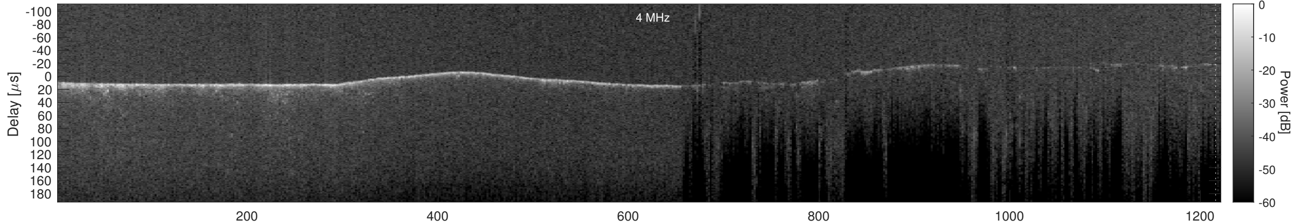
Orbit 7224, Cluttergram
