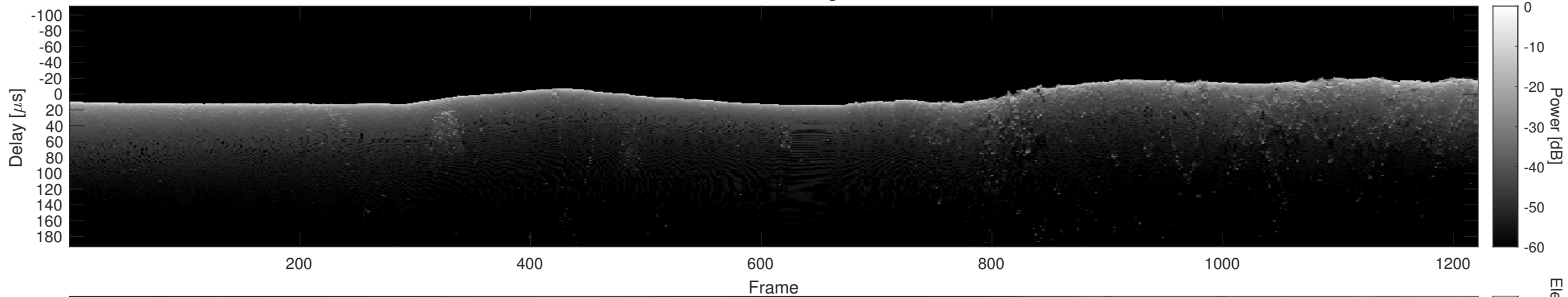
Orbit 7224, Cluttergram
