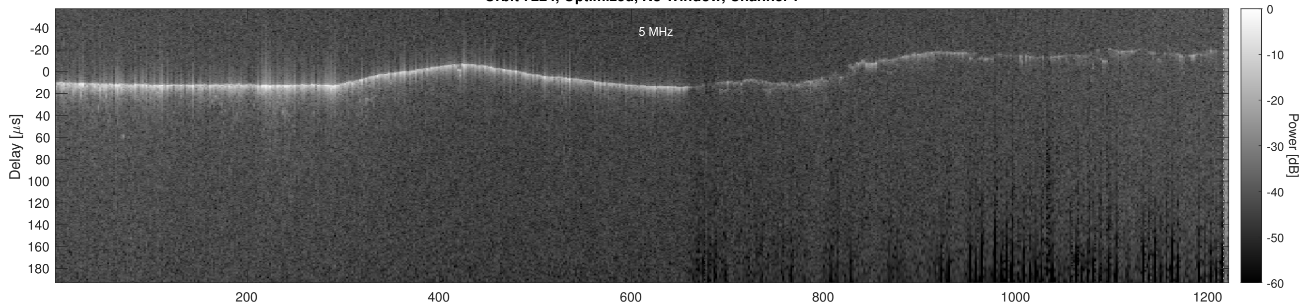
Orbit 7224, Optimized, No Window, Channel 2
