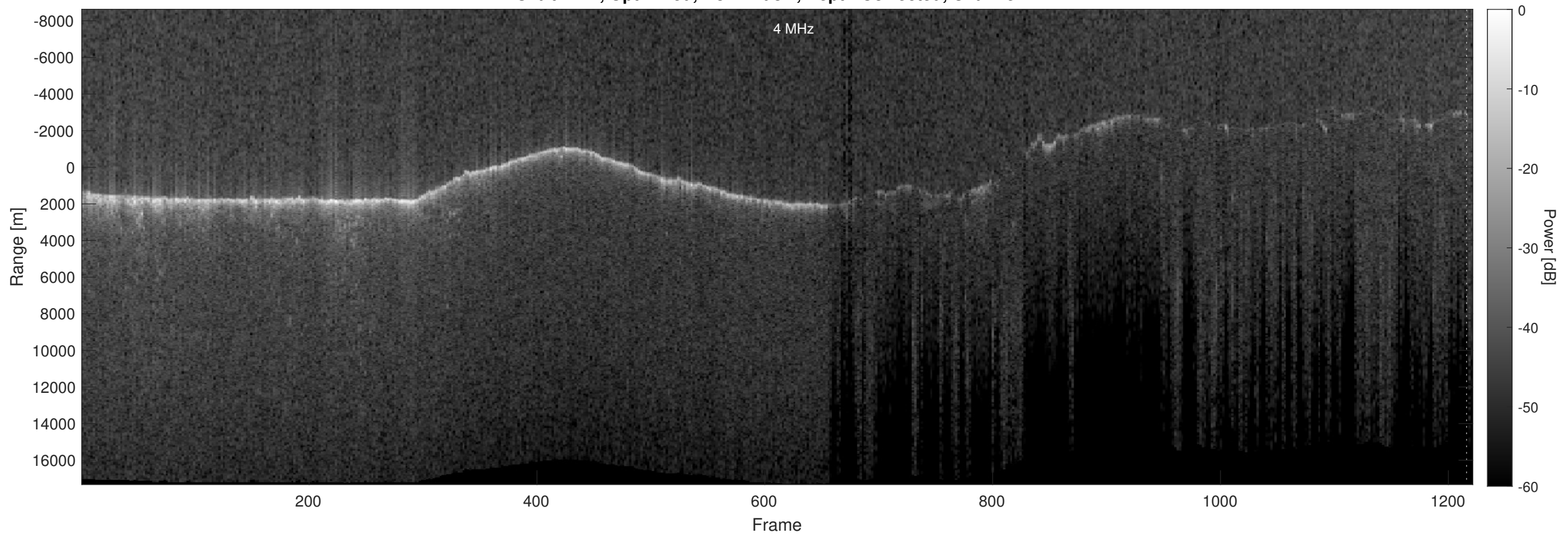
Orbit 7224, Optimized, No Window, Depth-Corrected, Channel 2
