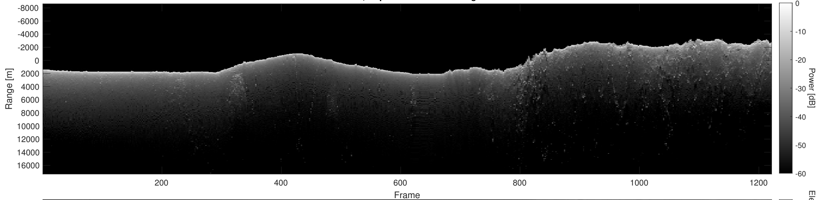
Orbit 7224, Depth-Corrected Cluttergram
