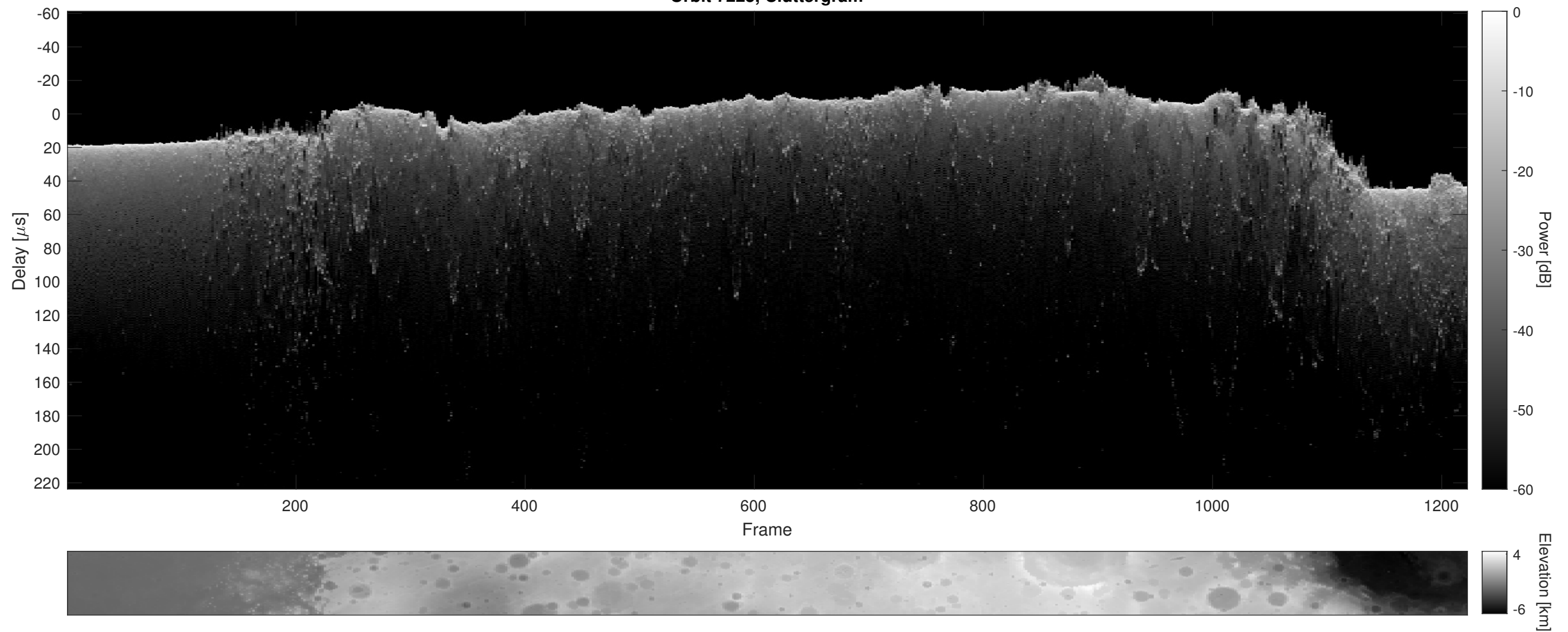
Orbit 7225, Cluttergram
