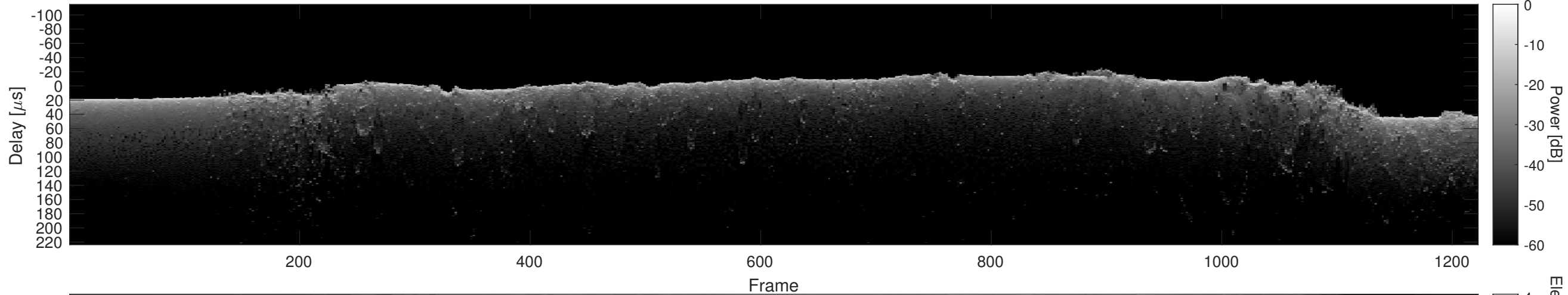
Orbit 7225, Cluttergram
