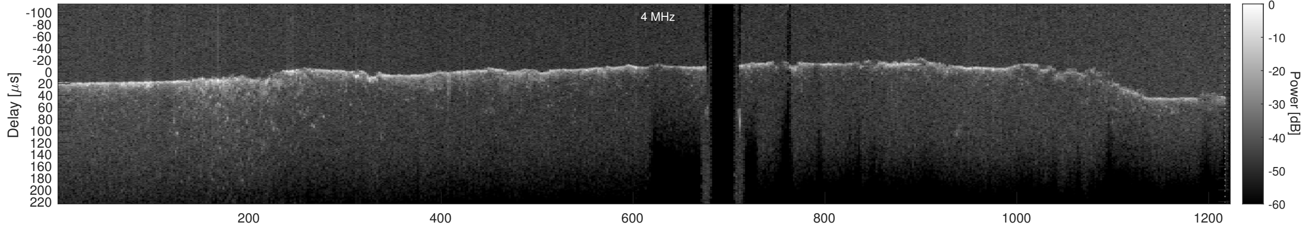
Orbit 7225, Cluttergram
