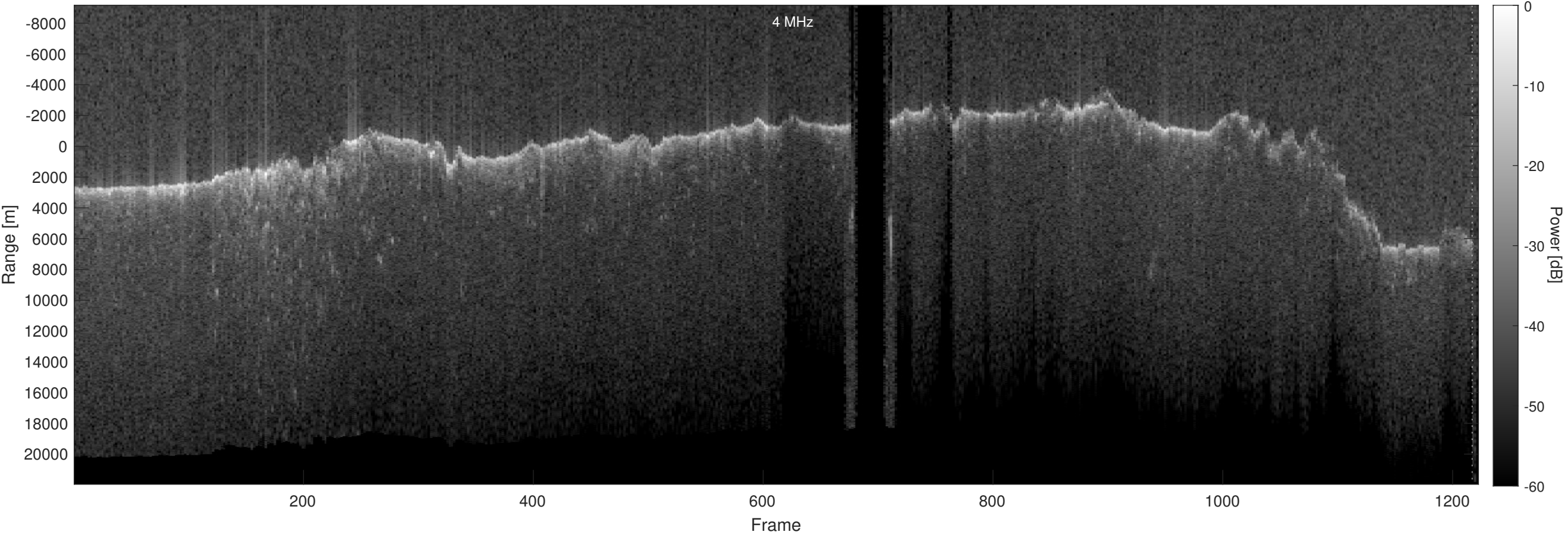
Orbit 7225, Optimized, No Window, Depth-Corrected, Channel 2
