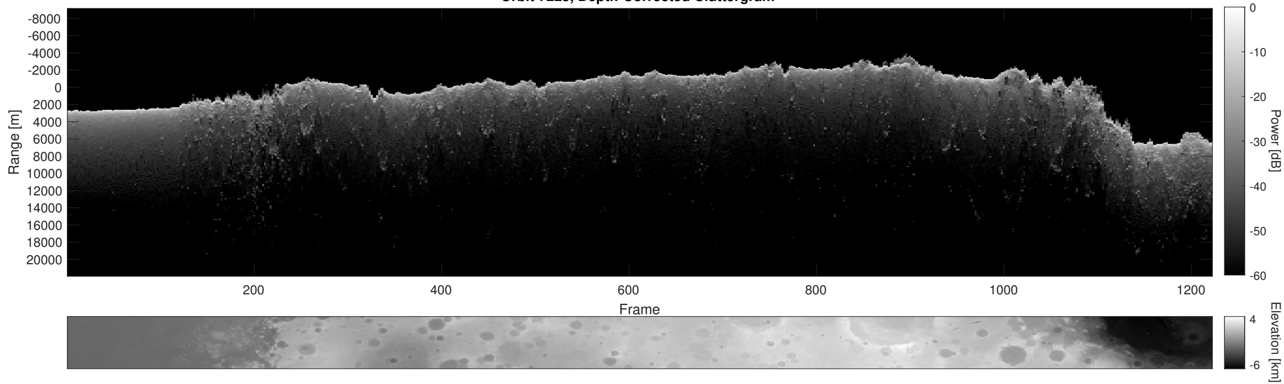
Orbit 7225, Depth-Corrected Cluttergram
