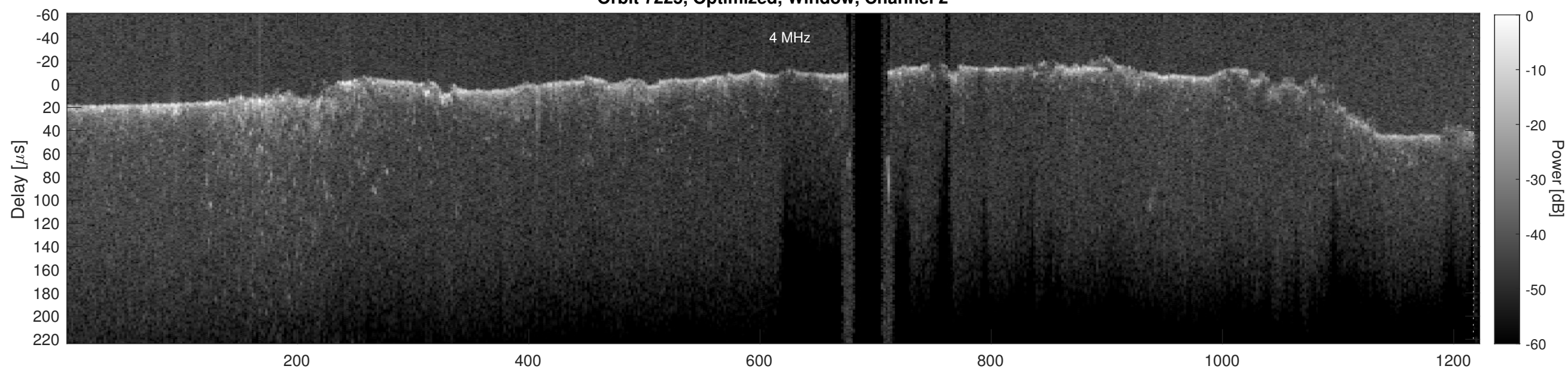
Orbit 7225, Cluttergram
