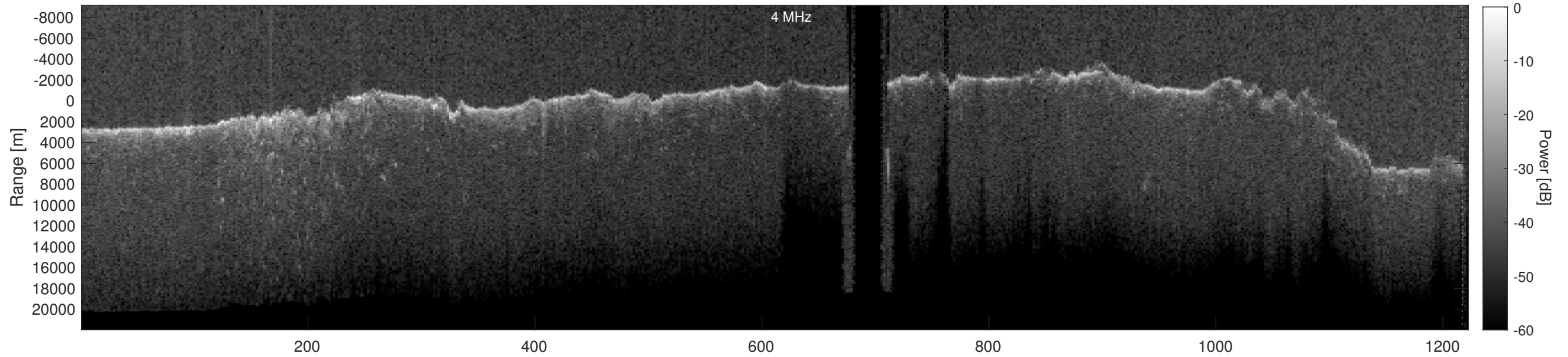
Orbit 7225, Depth-Corrected Cluttergram
