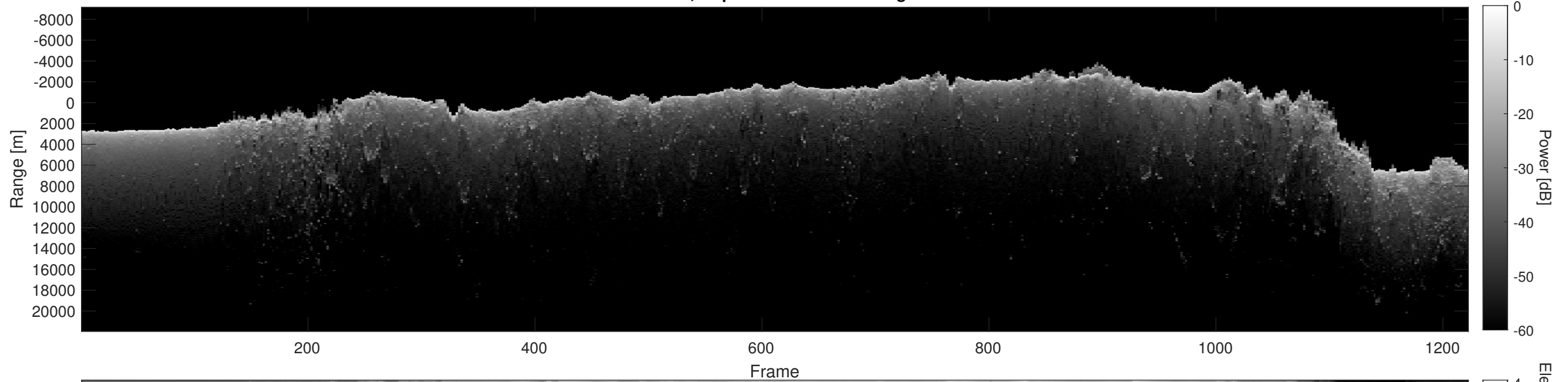
Orbit 7225, Depth-Corrected Cluttergram
