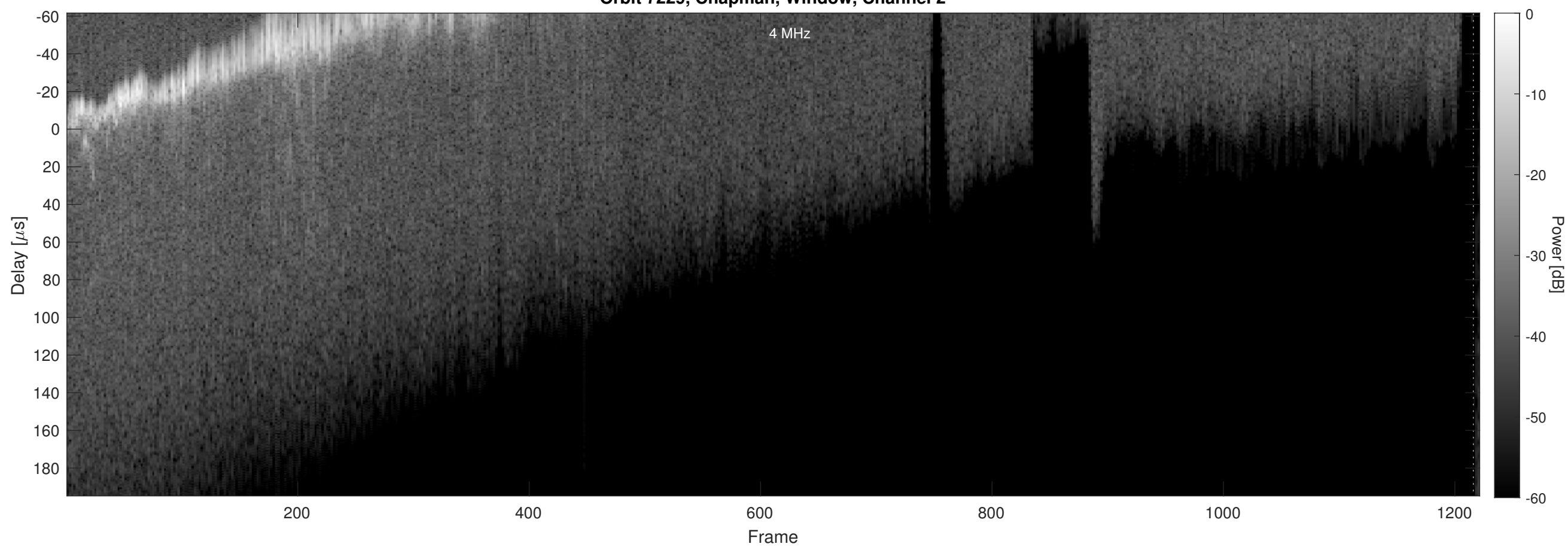
Orbit 7229, Chapman, Window, Channel 2
