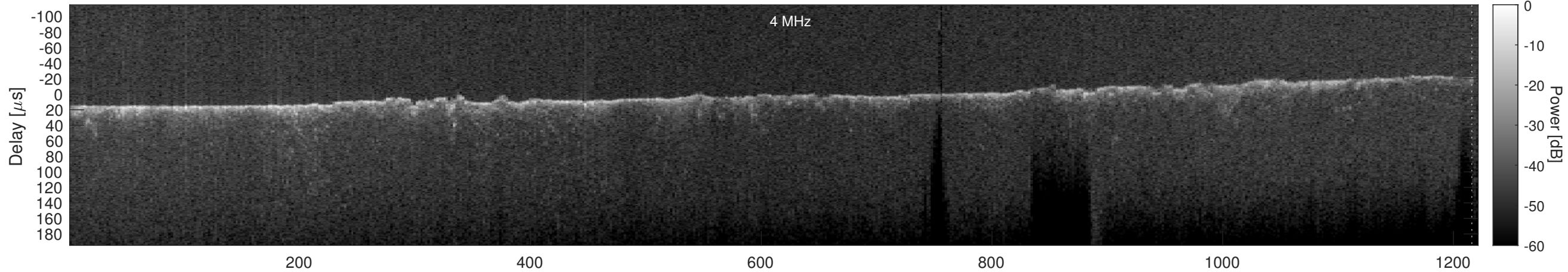
Orbit 7229, Cluttergram
