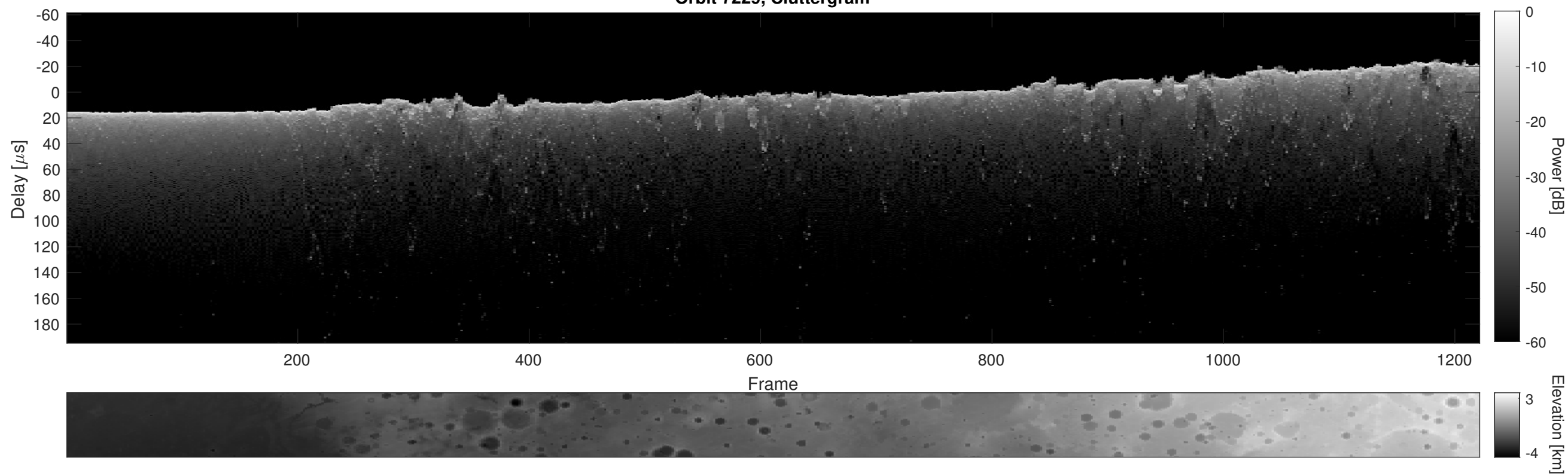
Orbit 7229, Cluttergram
