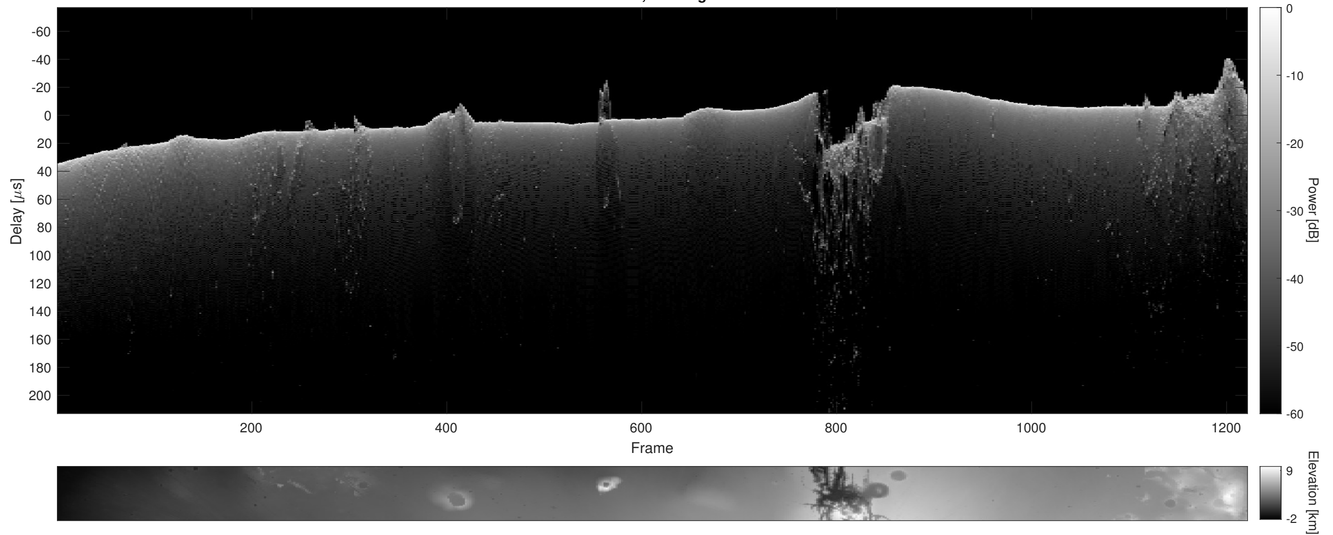
Orbit 7230, Cluttergram
