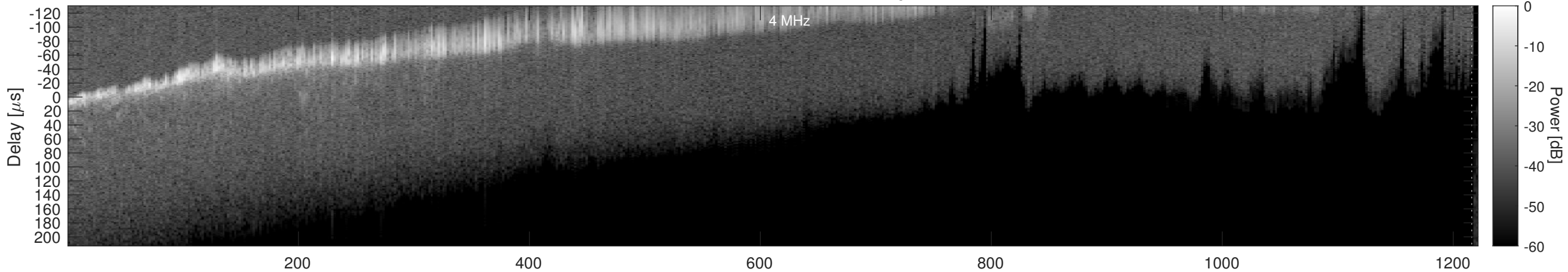
Orbit 7230, Window, Channel 2, Optimized
