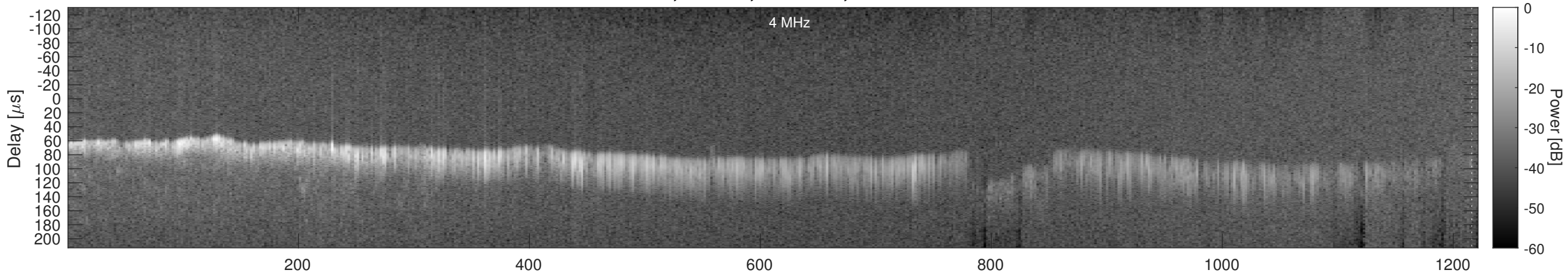
Orbit 7230, Window, Channel 2, Chapman
