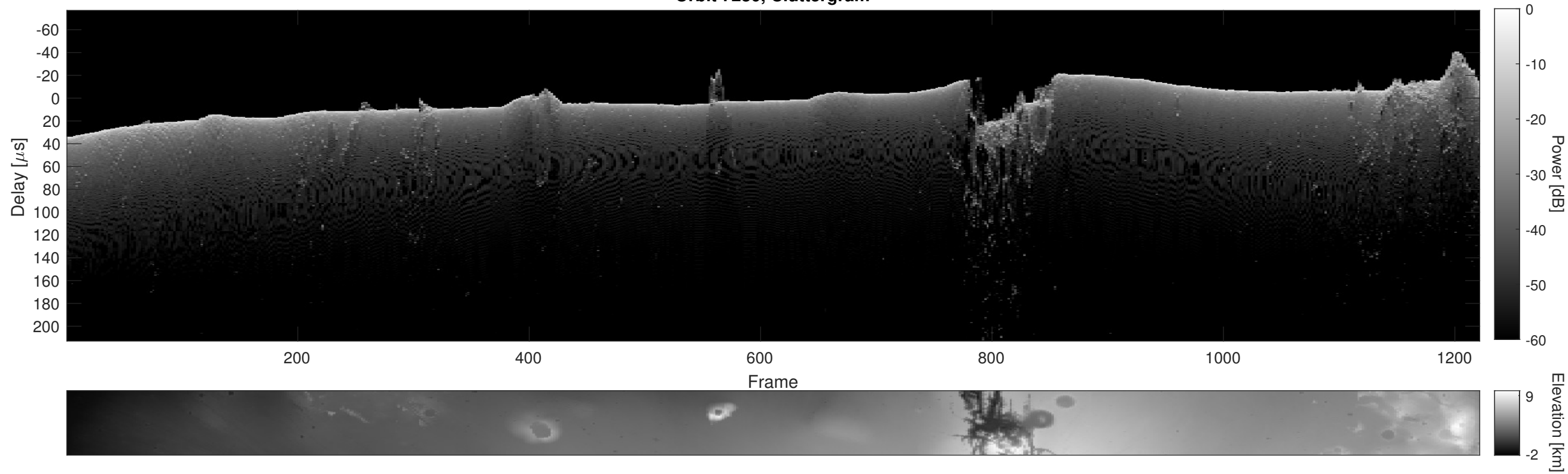
Orbit 7230, Cluttergram
