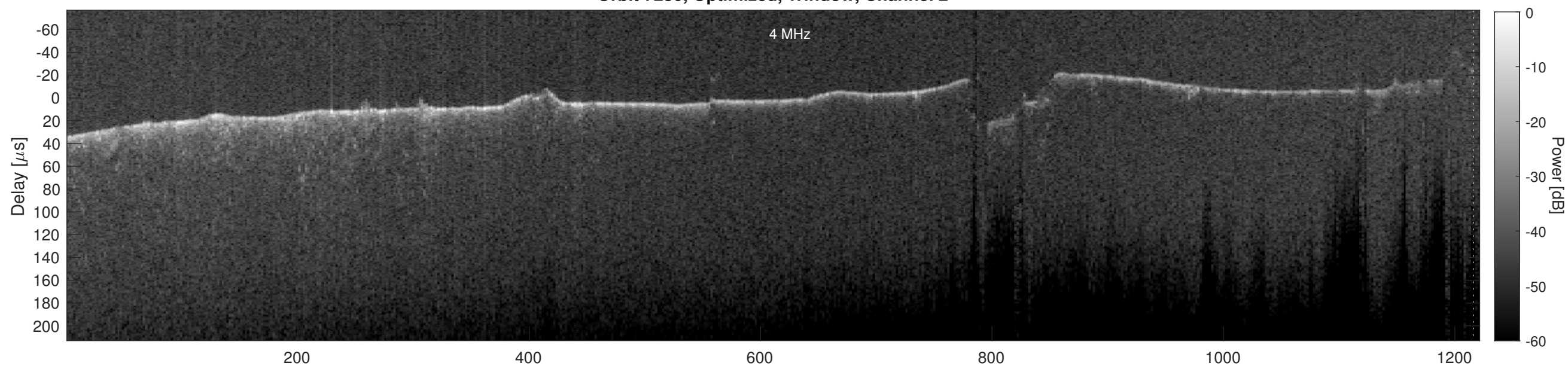
Orbit 7230, Cluttergram
