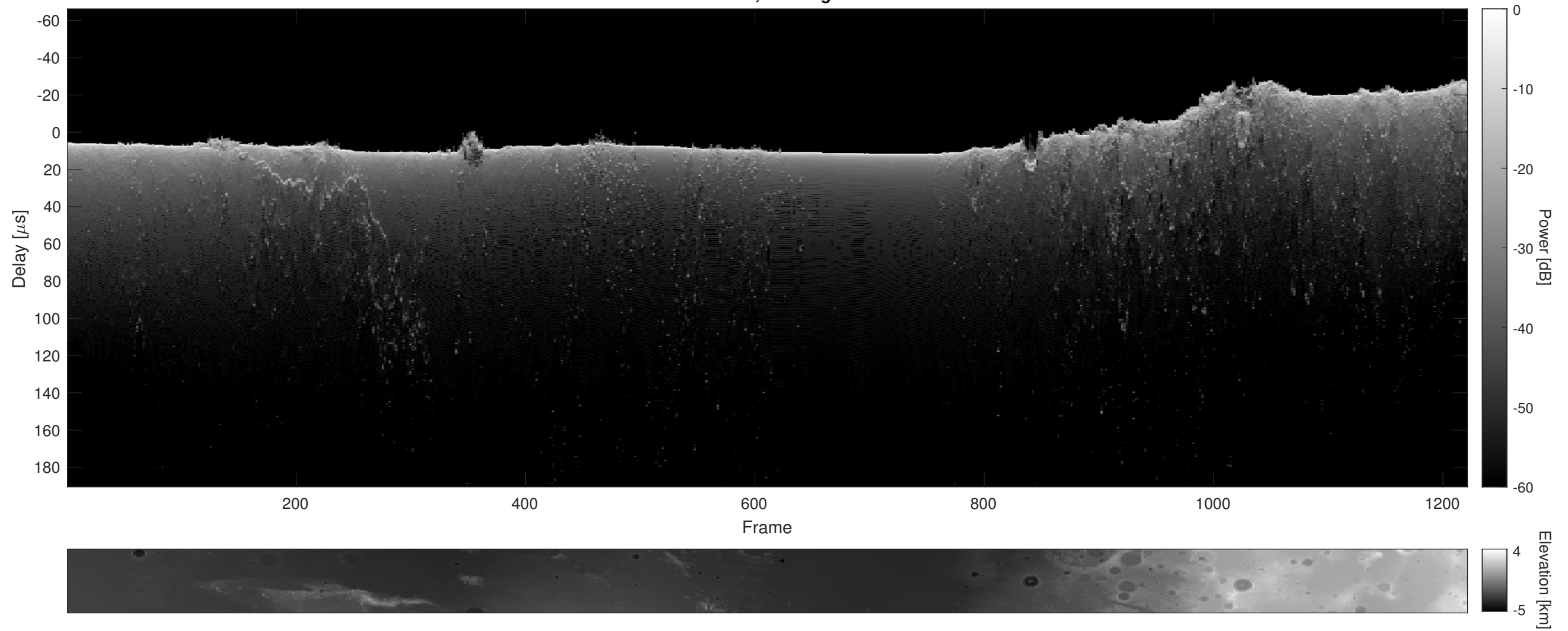
Orbit 7231, Cluttergram
