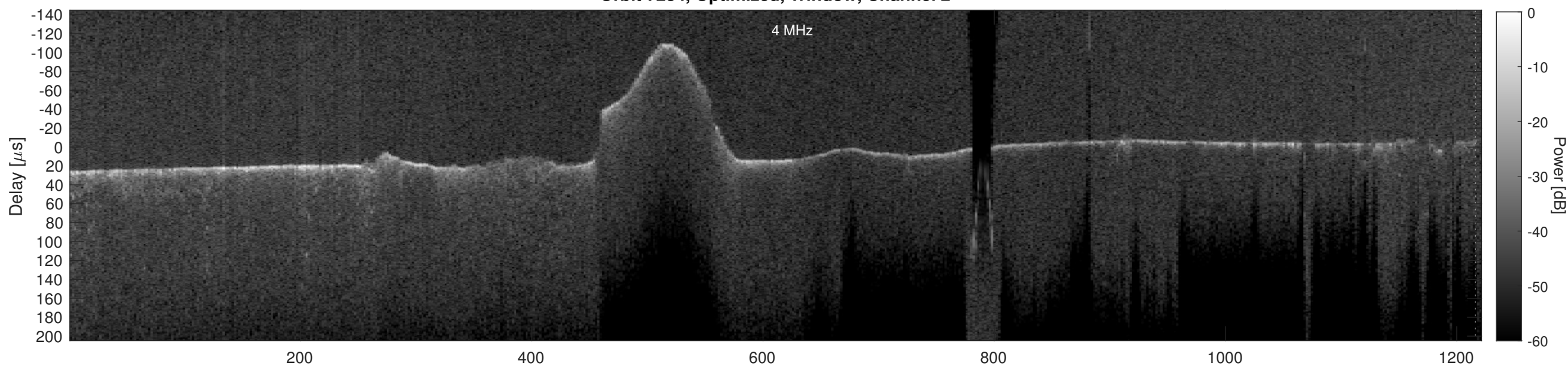
Orbit 7234, Cluttergram
