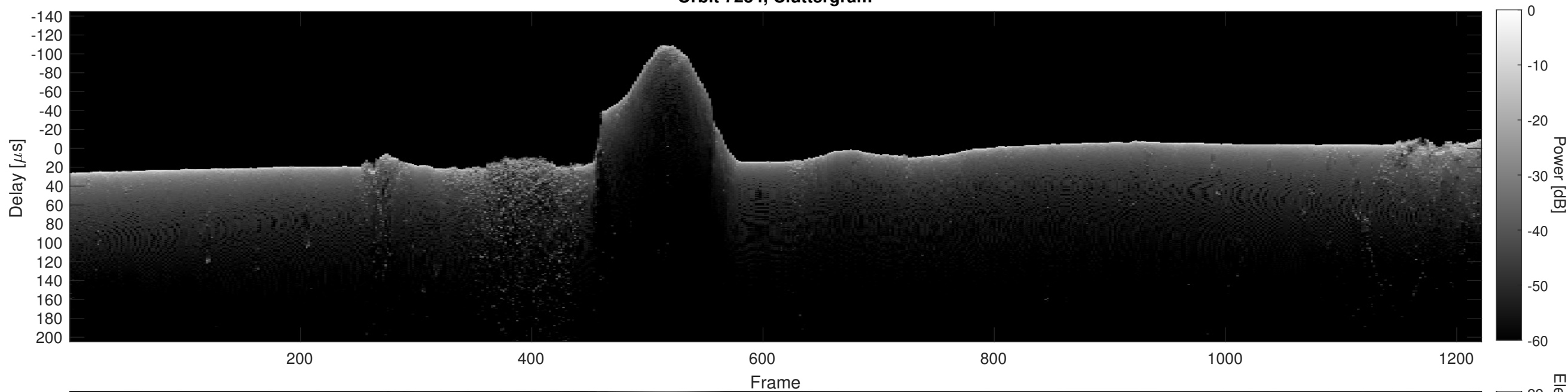
Orbit 7234, Cluttergram
