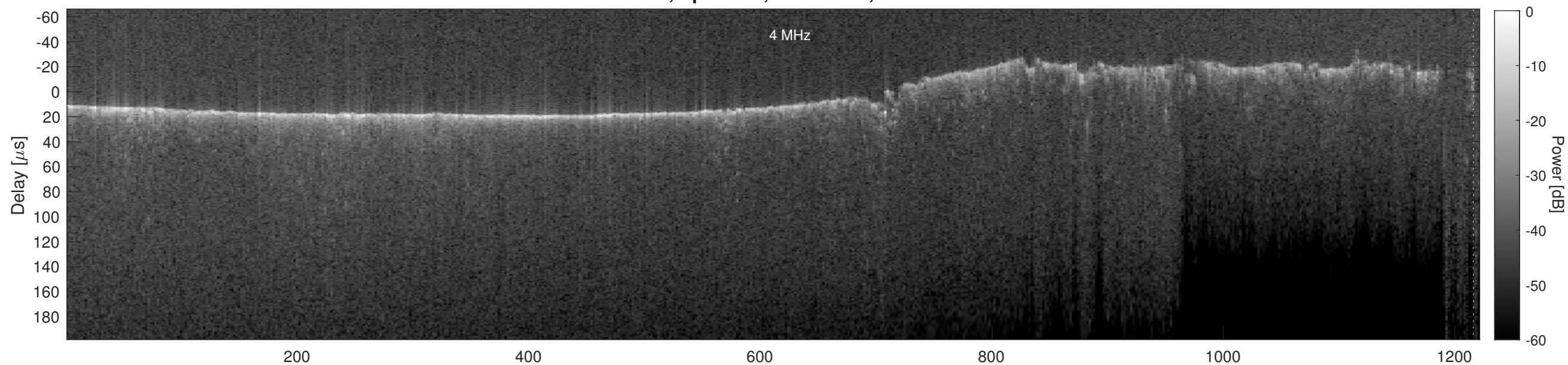
Orbit 7235, Cluttergram
