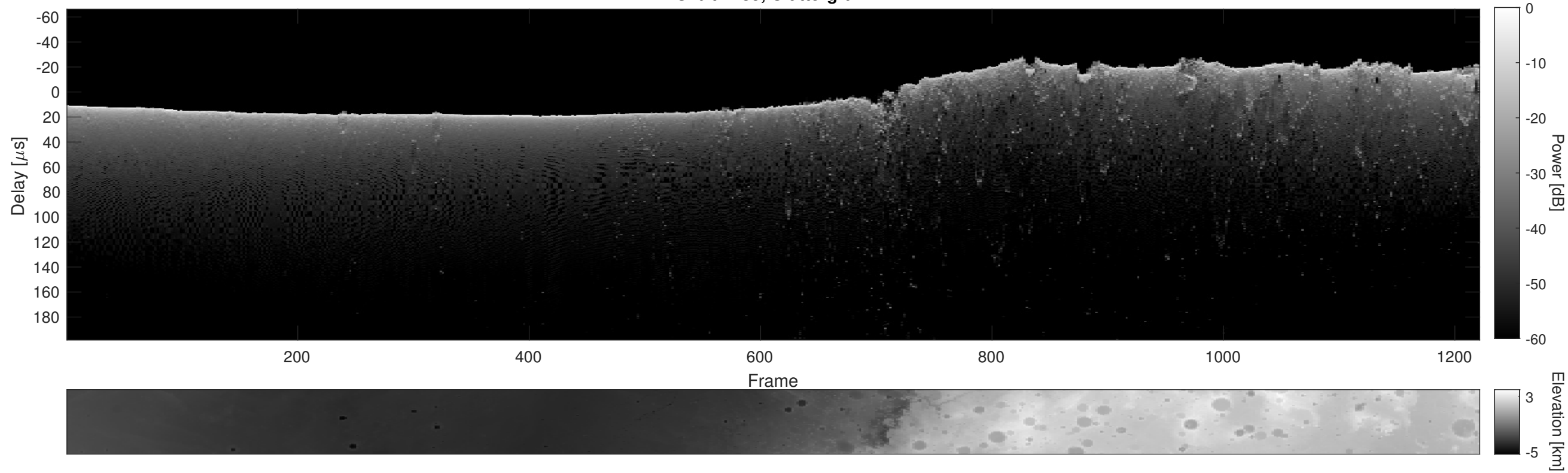
Orbit 7235, Cluttergram
