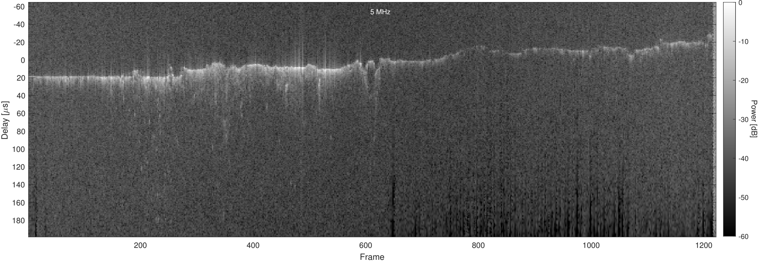
Orbit 7236, Optimized, No Window, Channel 2
