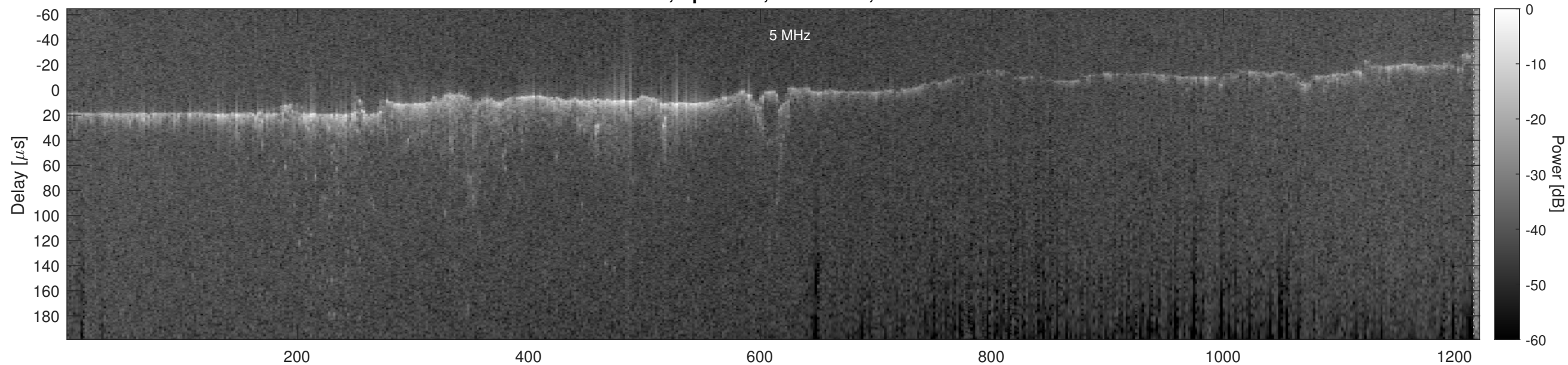
Orbit 7236, Optimized, No Window, Channel 2
