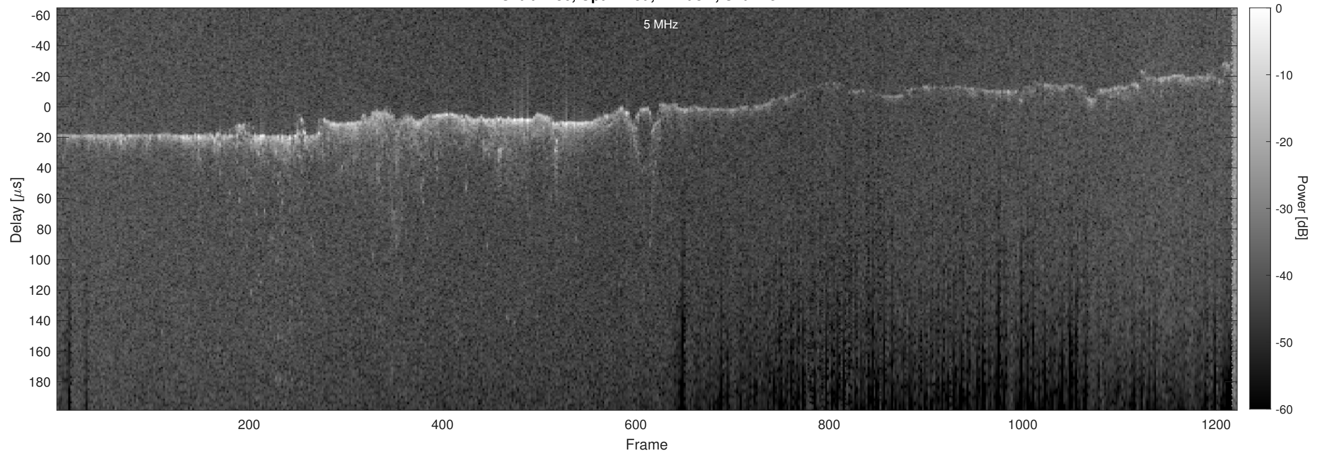
Orbit 7236, Optimized, Window, Channel 2
