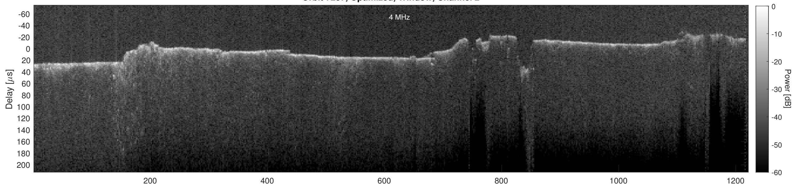
Orbit 7237, Cluttergram
