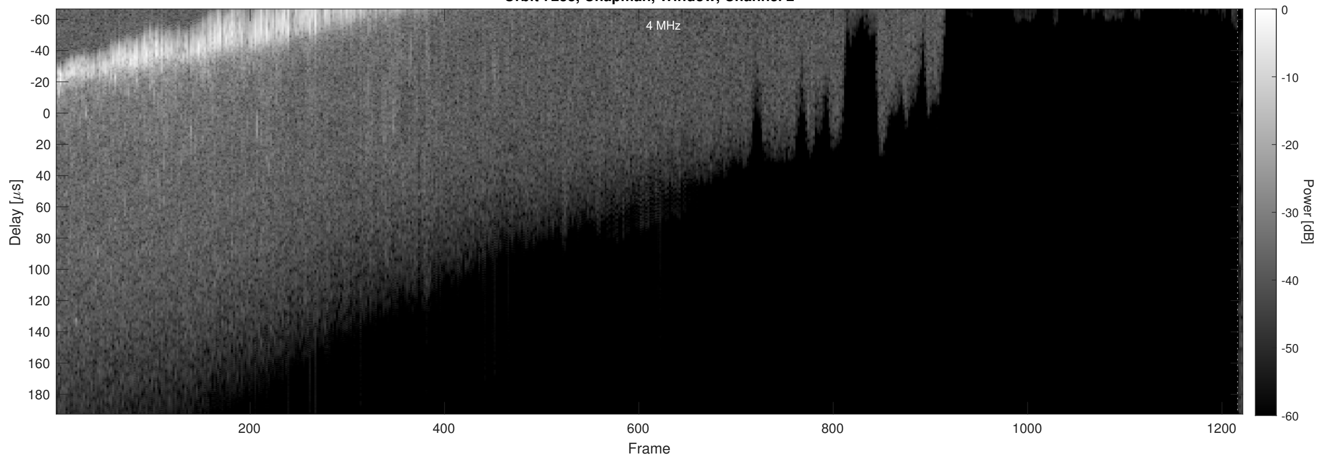
Orbit 7238, Chapman, Window, Channel 2
