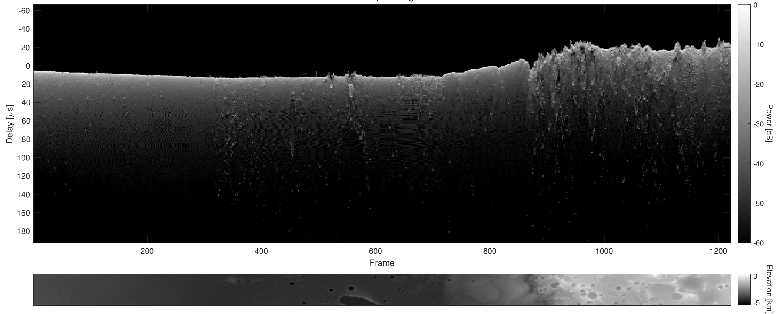
Orbit 7238, Cluttergram
