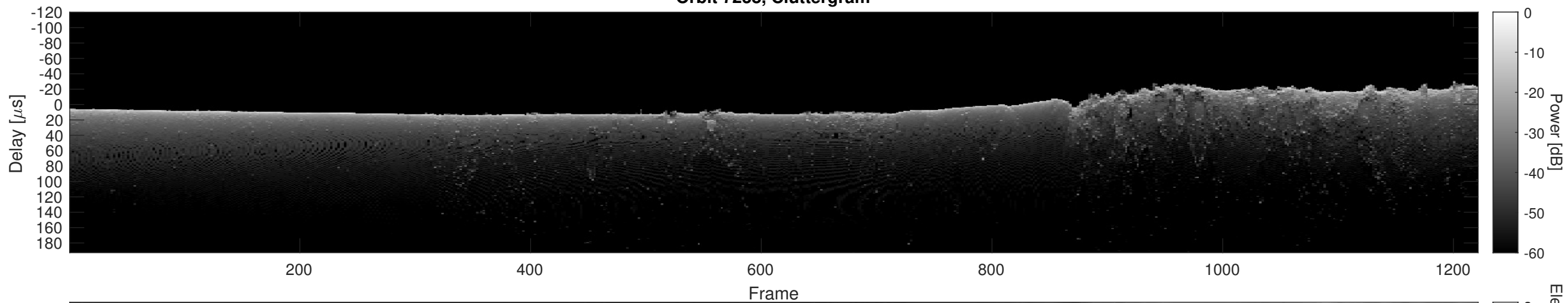
Orbit 7238, Cluttergram
