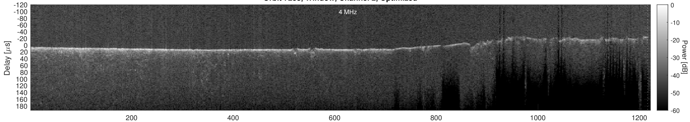
Orbit 7238, Cluttergram
