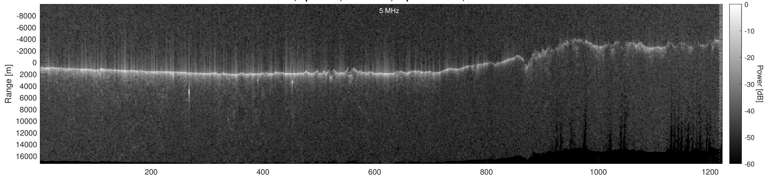
Orbit 7238, Optimized, No Window, Depth-Corrected, Channel 2
