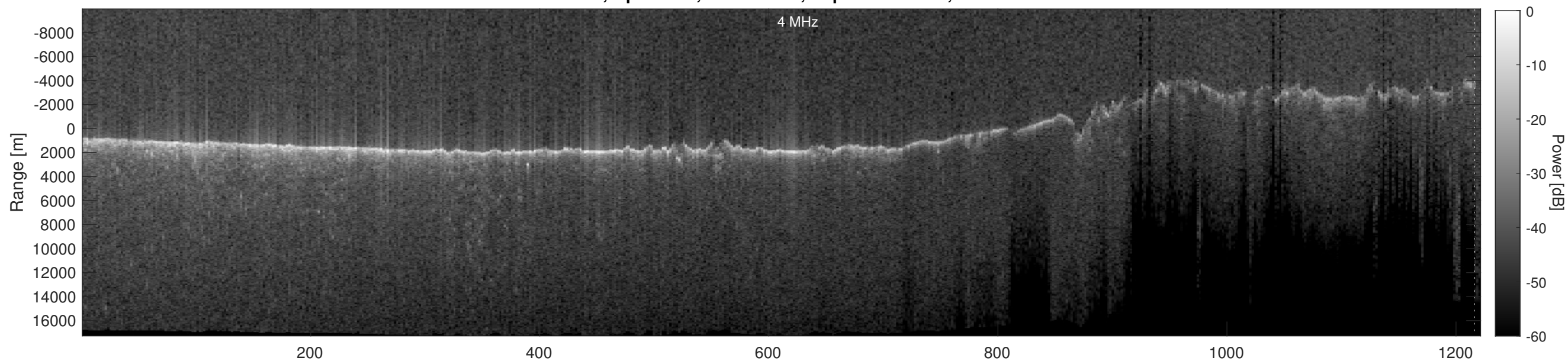
Orbit 7238, Depth-Corrected Cluttergram
