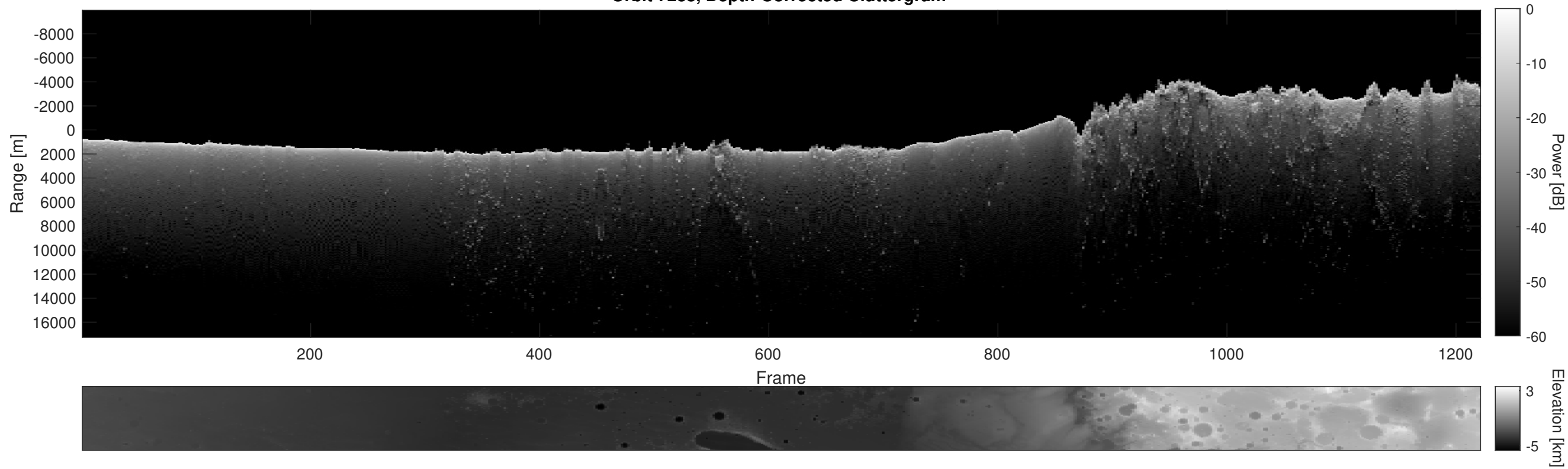
Orbit 7238, Depth-Corrected Cluttergram
