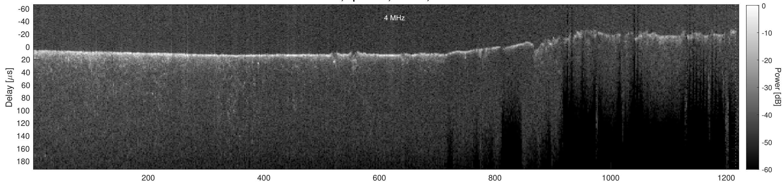
Orbit 7238, Cluttergram
