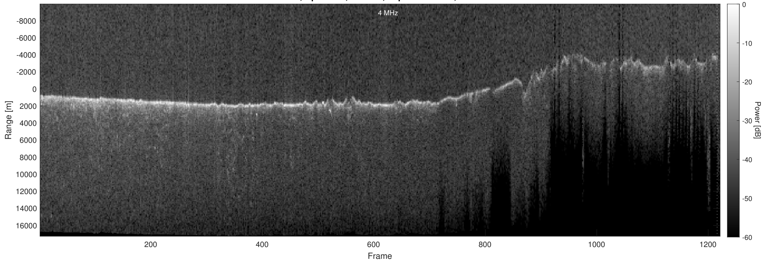
Orbit 7238, Optimized, Window, Depth-Corrected, Channel 2
