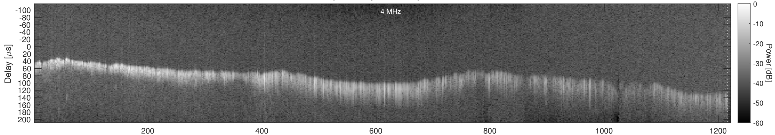
Orbit 7239, Window, Channel 2, Chapman
