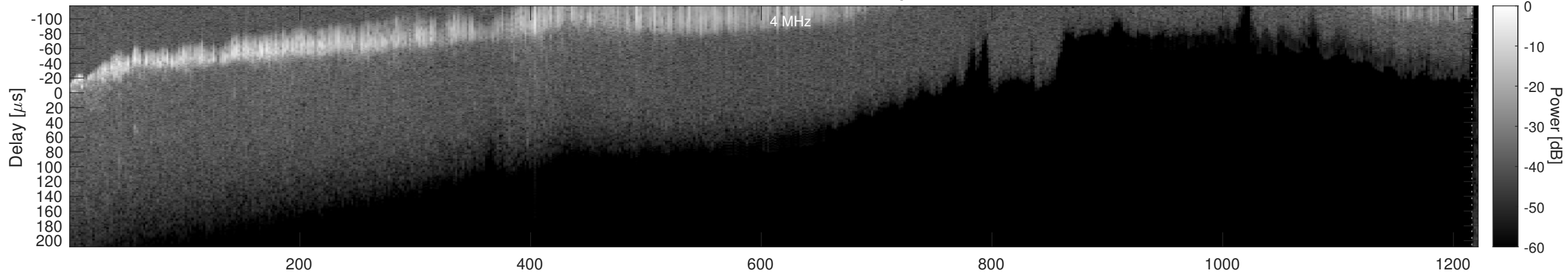
Orbit 7239, Window, Channel 2, Optimized
