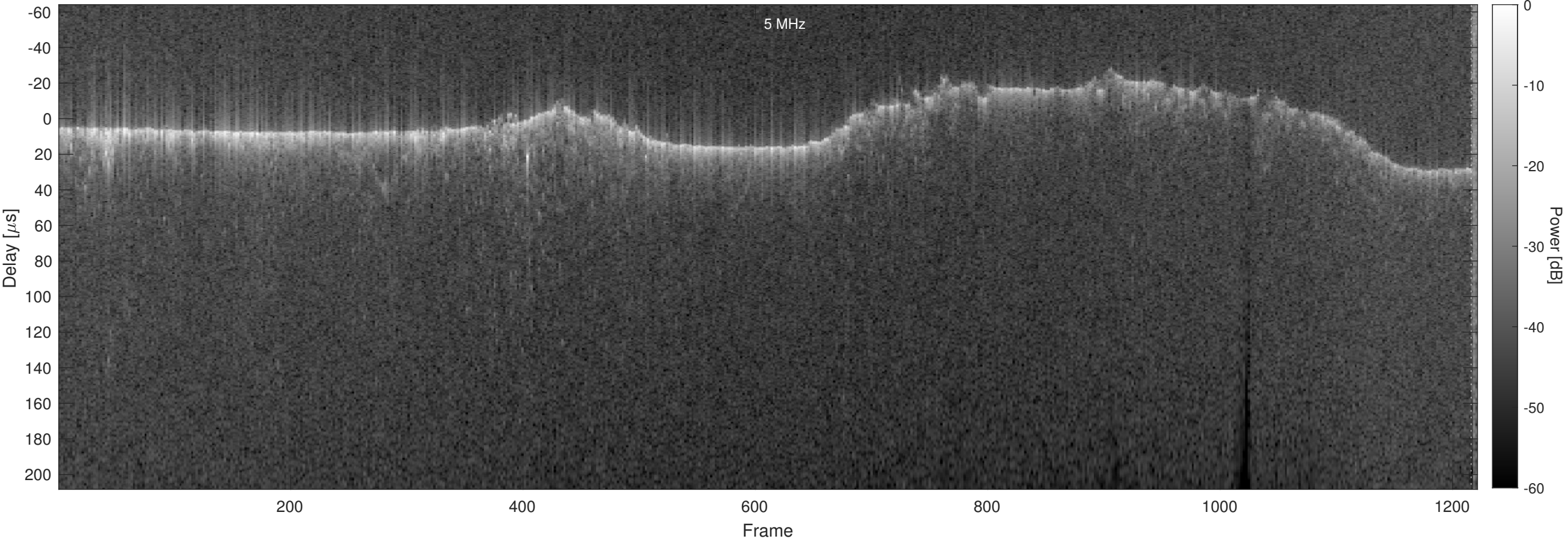
Orbit 7239, Optimized, No Window, Channel 2
