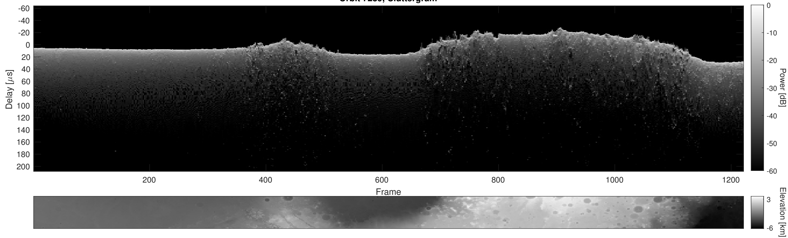
Orbit 7239, Cluttergram
