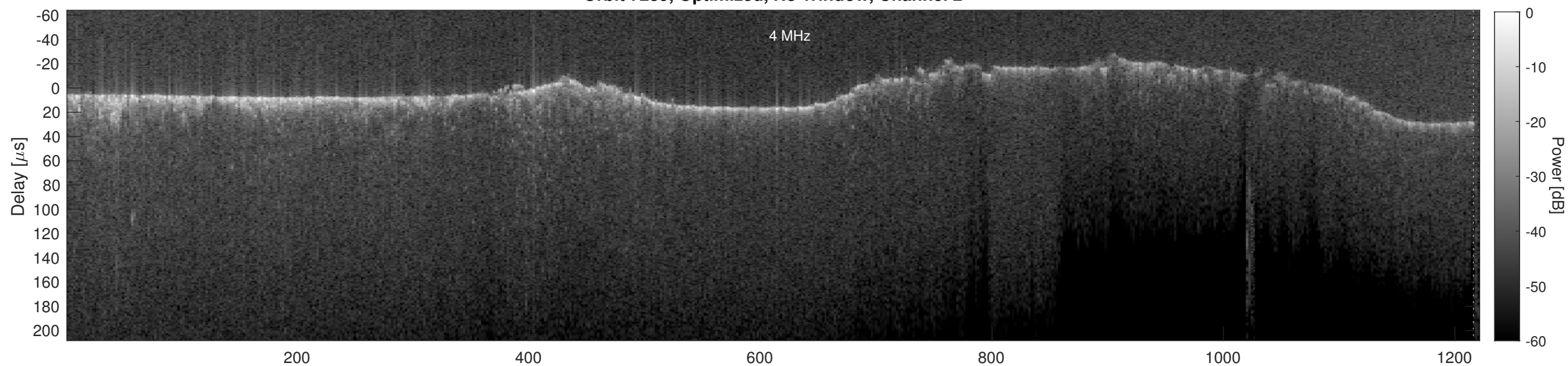
Orbit 7239, Cluttergram
