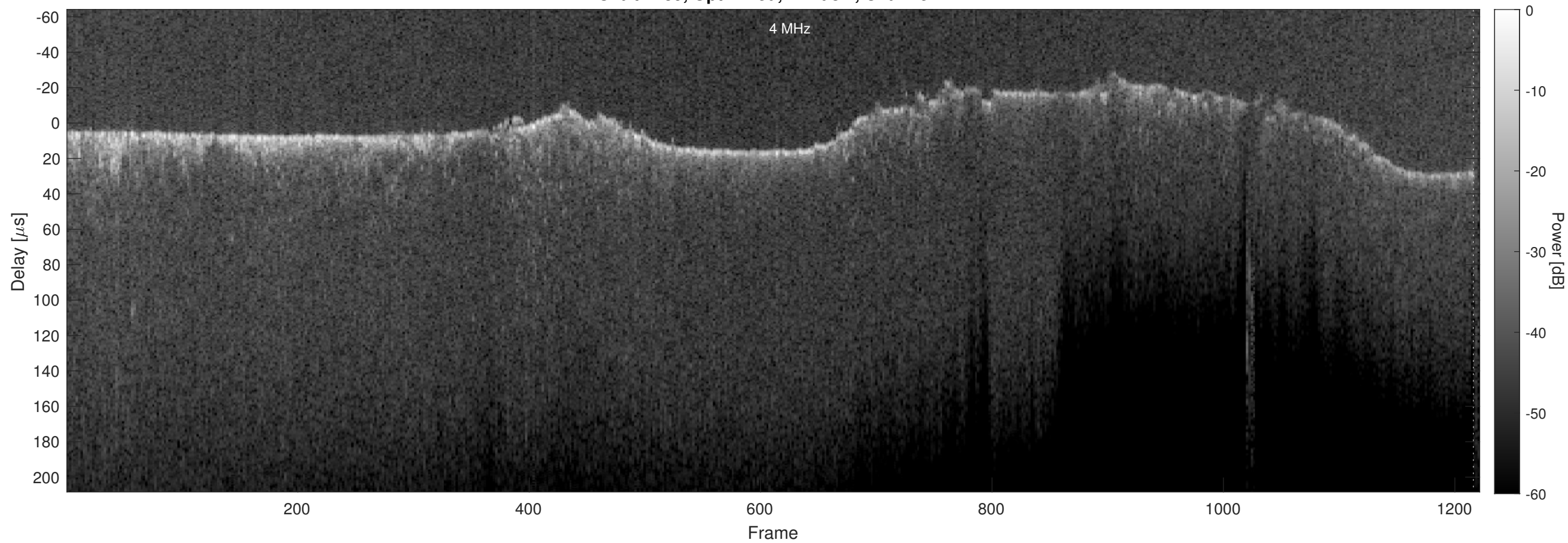
Orbit 7239, Optimized, Window, Channel 2
