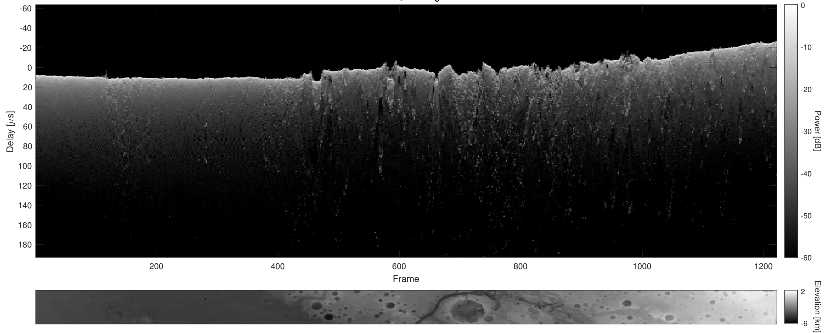
Orbit 7240, Cluttergram
