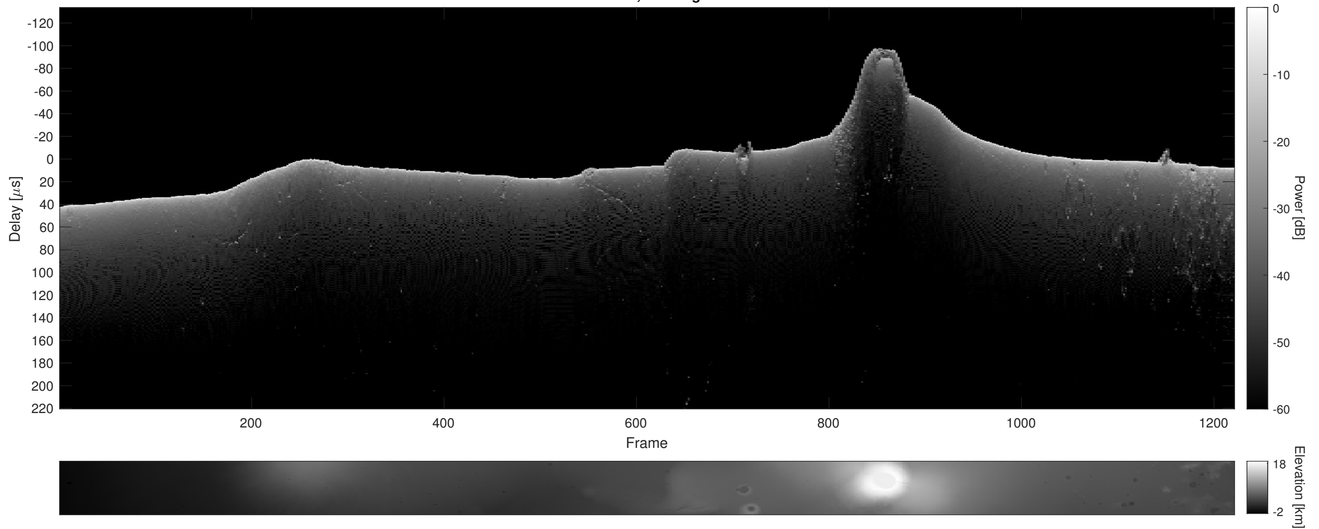
Orbit 7241, Cluttergram
